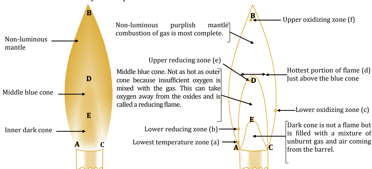
Fig. : Zones of flame of Bunsen burner
