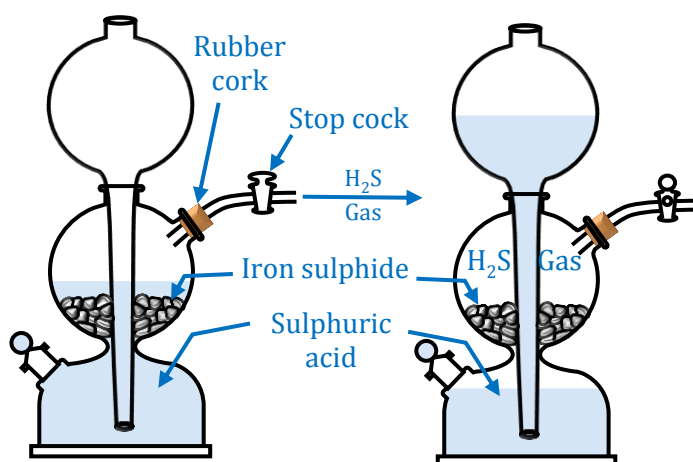
Fig. : Kipp's apparatus for preparation of \text{H}_2\text{S} gas
