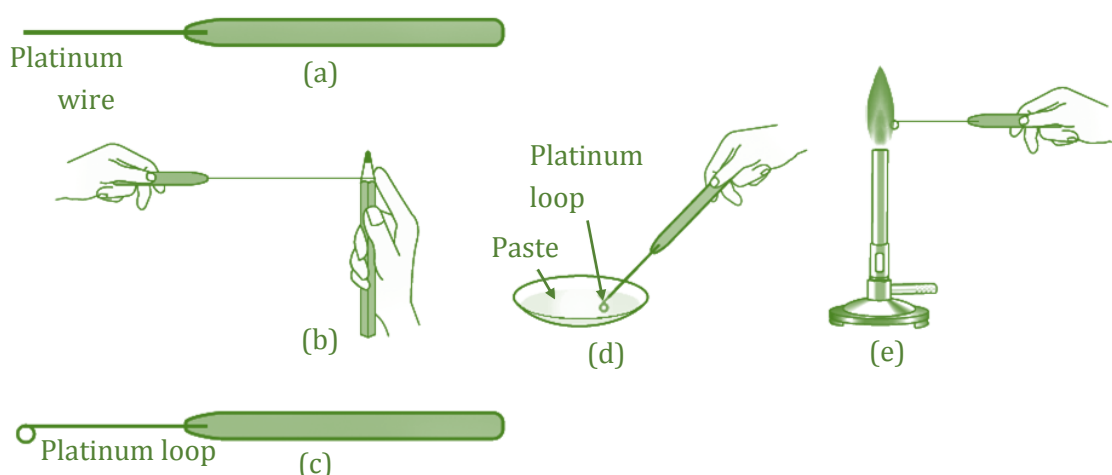
Fig. : Performing flame test
