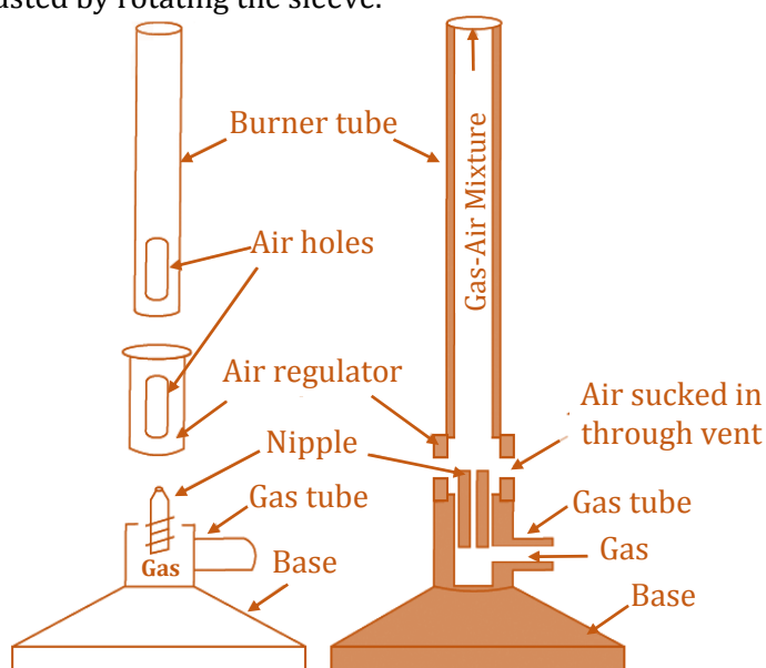
Fig. : Parts of Bunsen burner
