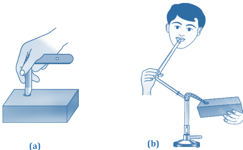
Fig. : (a) Making charcoal cavity
