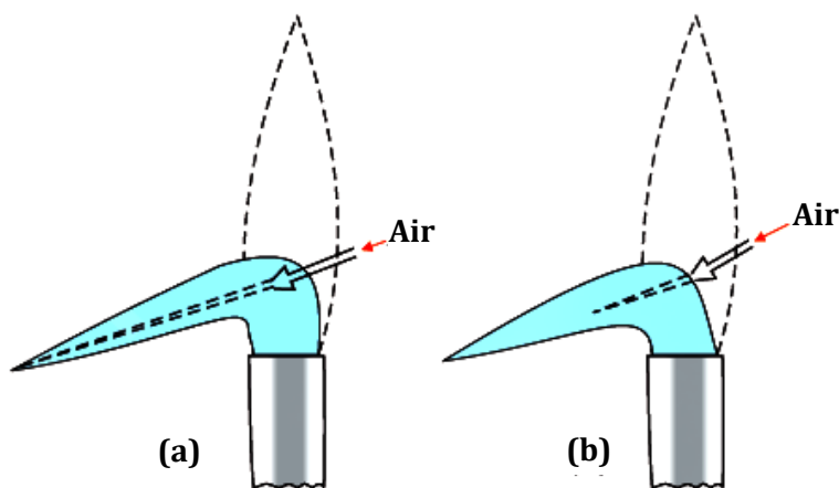
Fig. : Obtaining oxidizing and reducing flame (a) Oxidizing flame; and (b) Reducing flame
